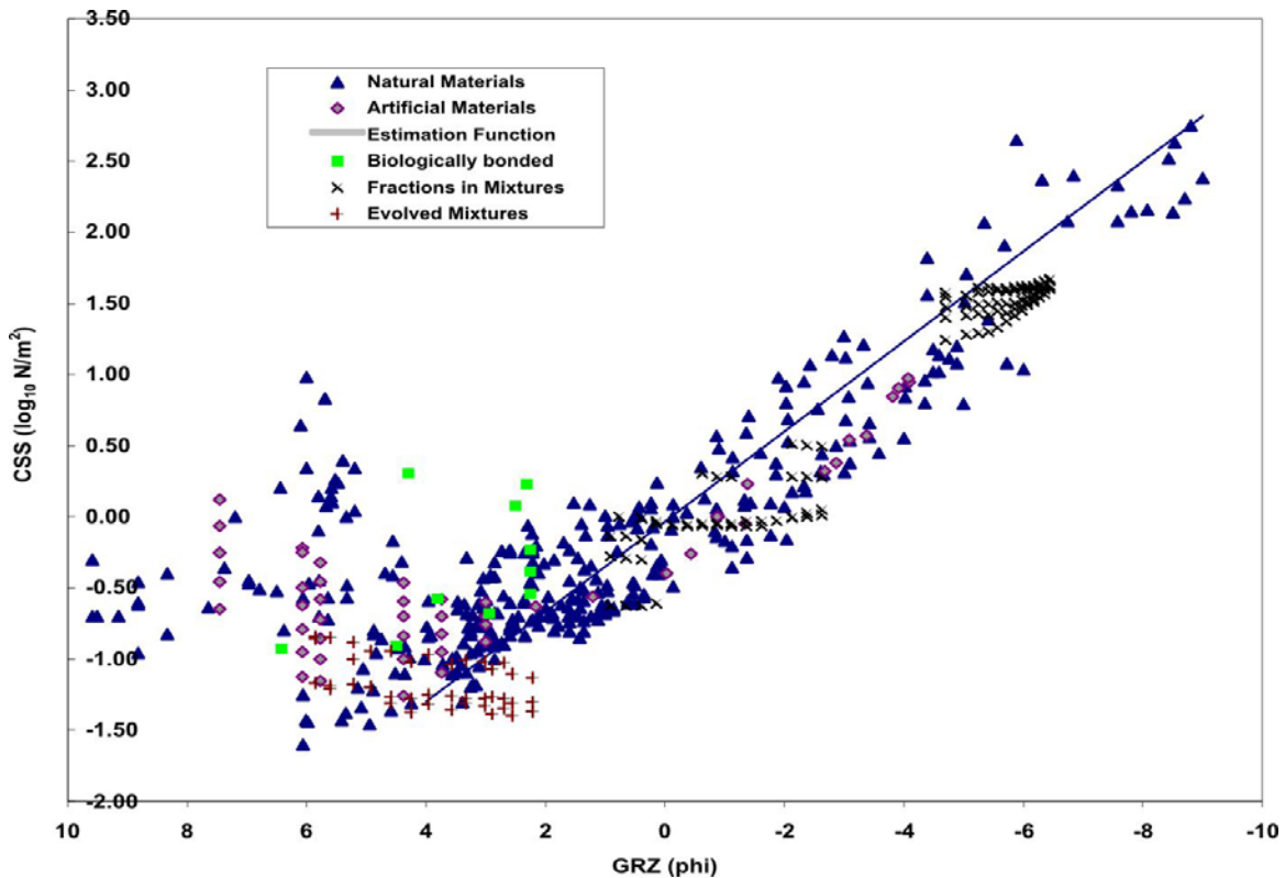
Fig. 3. A compilation of Critical Shear Stress results by sediment grain size over the gravel to clay range. Over 24 references were used referring to marine and river sediments, field and laboratory experiments, on unaltered and manipulated natural sediments.
