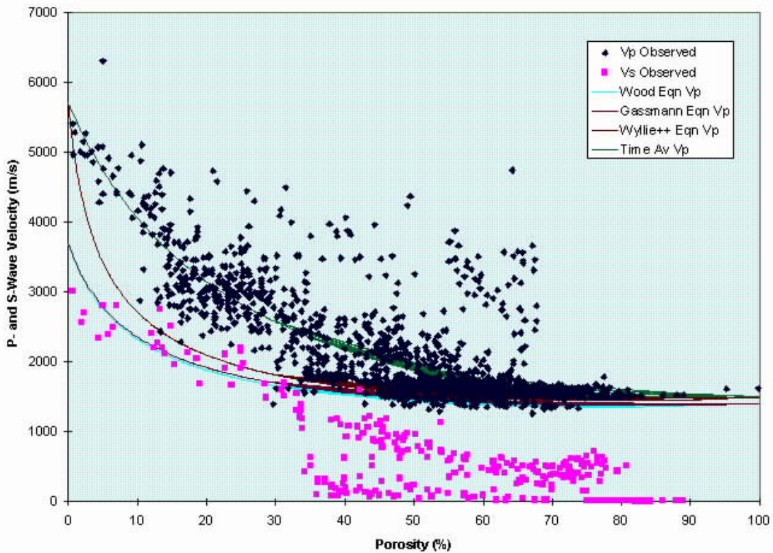
Fig. 1. The distribution of sediments by their Porosity and P- and S-wave Velocity values. Several separate populations are apparent. For P-wave velocities, the loose sediments with low velocities from 34% porosity and following the Gassman function; consolidated sediments following the Time-average relation; apparently cemented sediments with anomalously high velocities for the porosity. The S-wave populations have yet to be explained.
